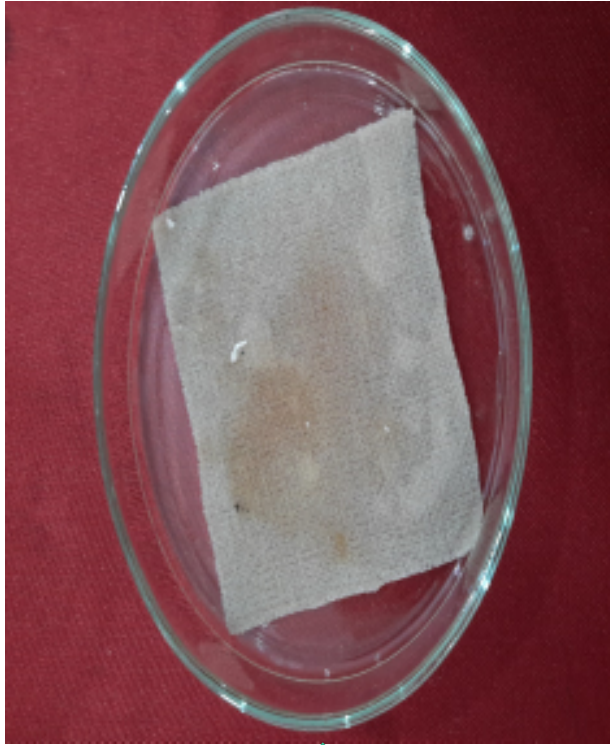
NaOH
